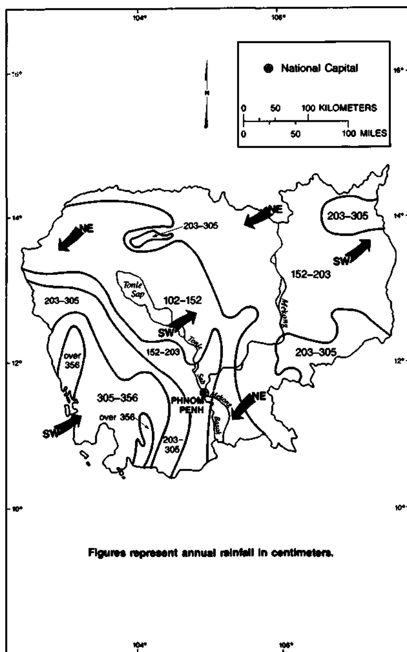
Figure 5. Annual Rainfall and Monsoon Airflow
